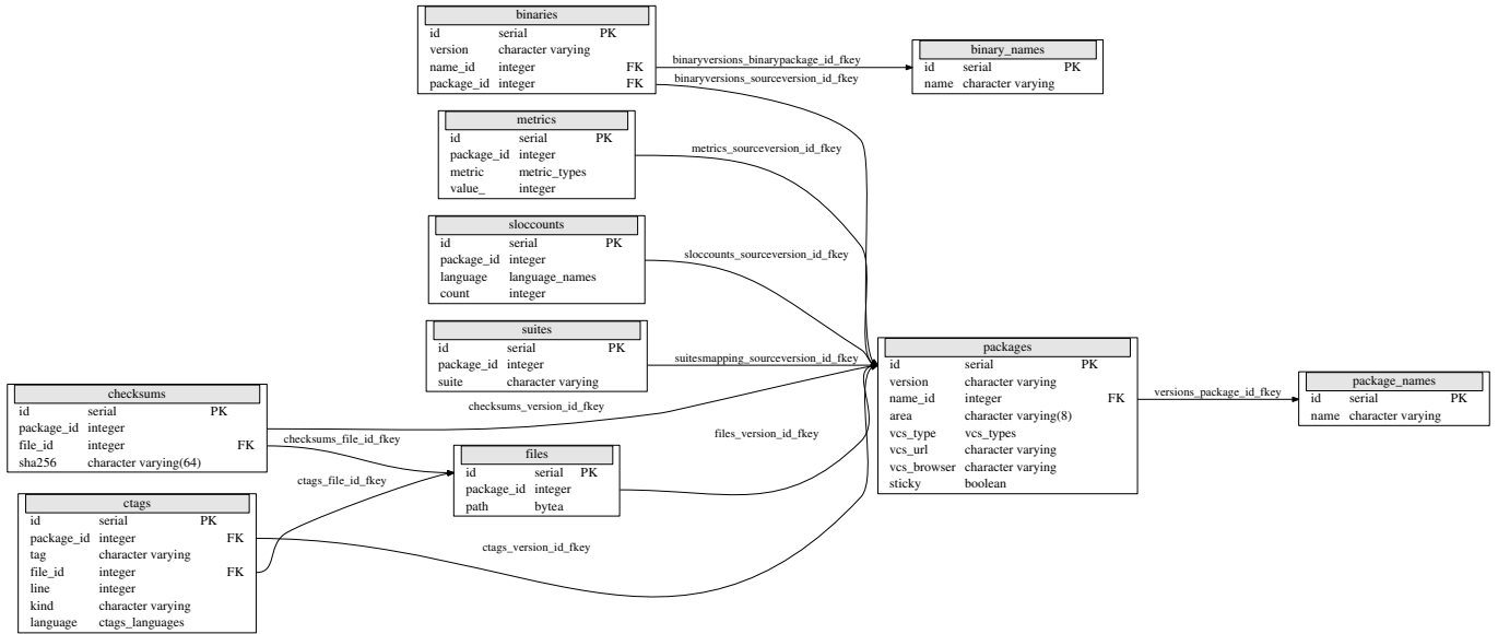
Fig. 1. Debsources DB schema, part 1: main tables
