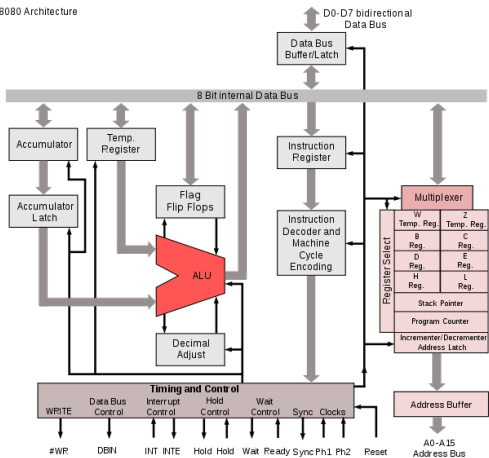
Intel 8080 Architecture
