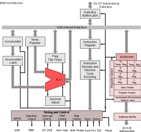
Intel 8080 Architecture
